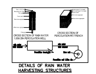
DETAILS OF RAIN WATER HARVESTING STRUCTURES
